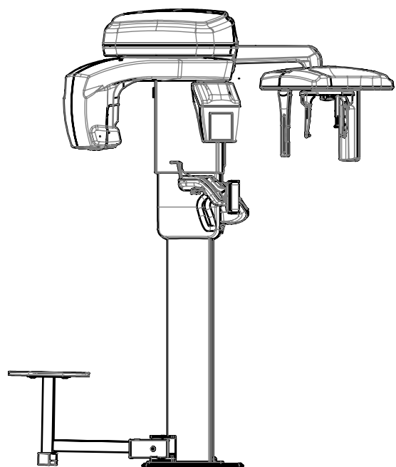
CS9600wt SC Scale 1:30
